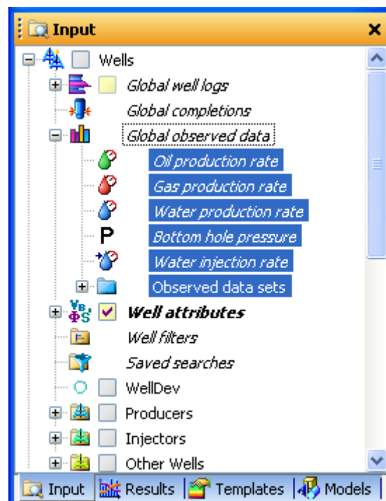
Fig.26.4: Global observed data after adding
